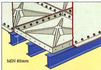
OPTION 3. FULL-SPAN BASE - INTERNALLY BOLTED BASE PANELS. @ 1000mm centres
