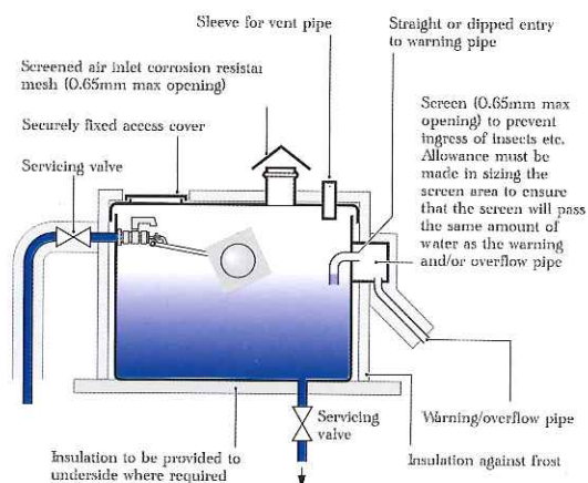
Principal details of a cistern storing water 儲水箱安裝完成圖(參考圖)
