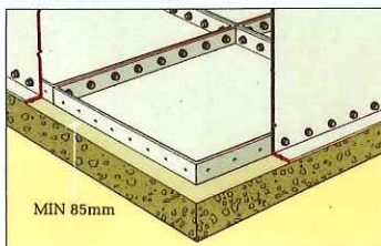
OPTION 2. HALF-SPAN BASE - INTERNALLY BOLTED BASE PANELS. @ 500mm centres
