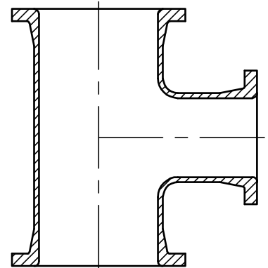
Flanged Tee
