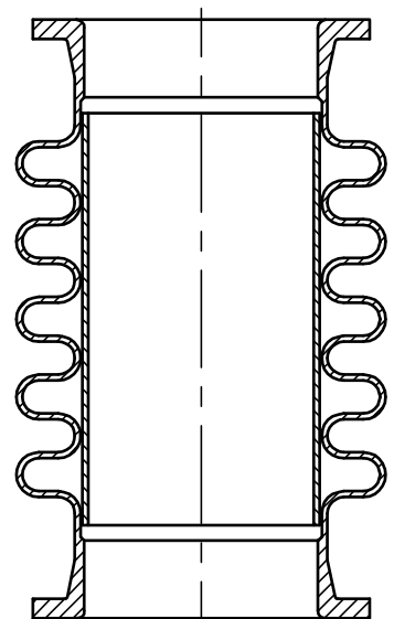
Flanged Bellow
